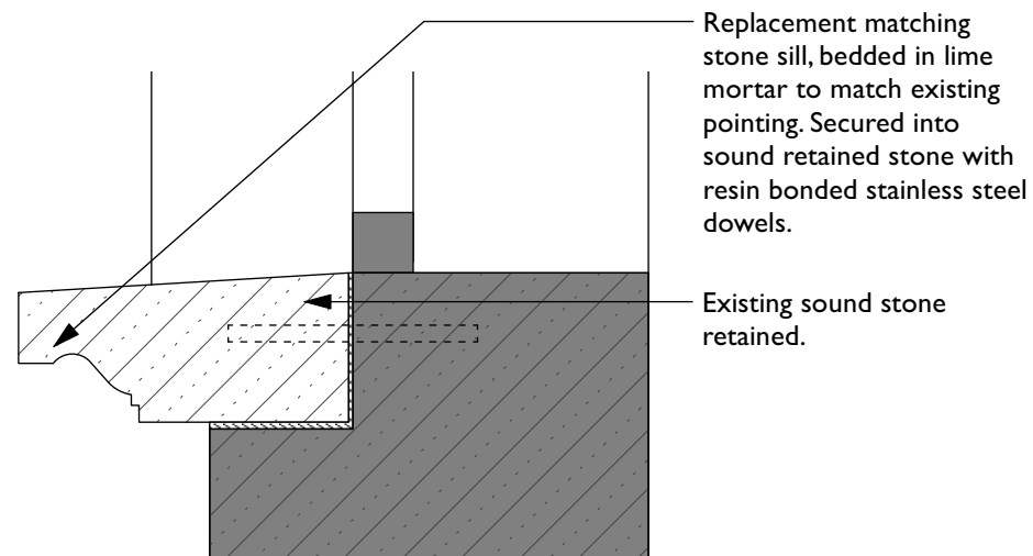
1 Typical Stone Reinstatement Detail Scale: 1:10
