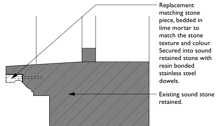
3 Typical Stone Reinstatement Detail Scale: 1:10
