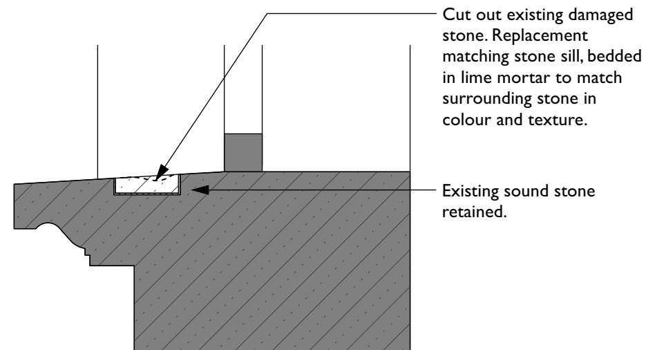
2 Typical Stone Reinstatement Detail Scale: 1:10
