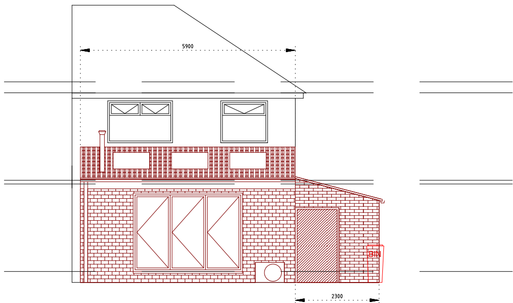
REAR ELEVATION (A3 1:100)
