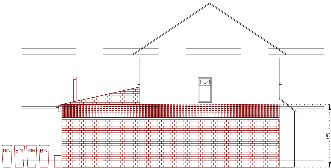
SIDE ELEVATION ELEVATION (from No.6)(A3 1:100)
