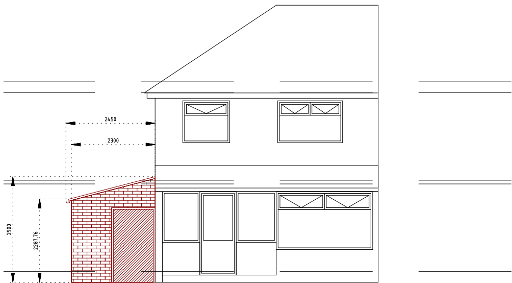
FRONT ELEVATION (A3 1:100)
