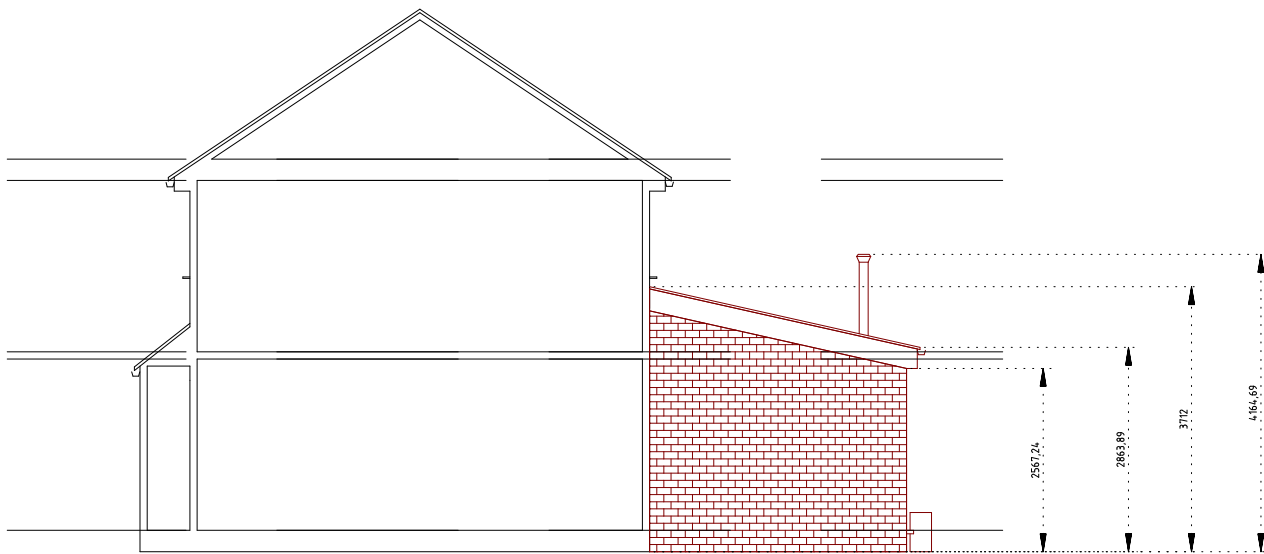
SIDE ELEVATION ELEVATION (from No.2)(A3 1:100)
