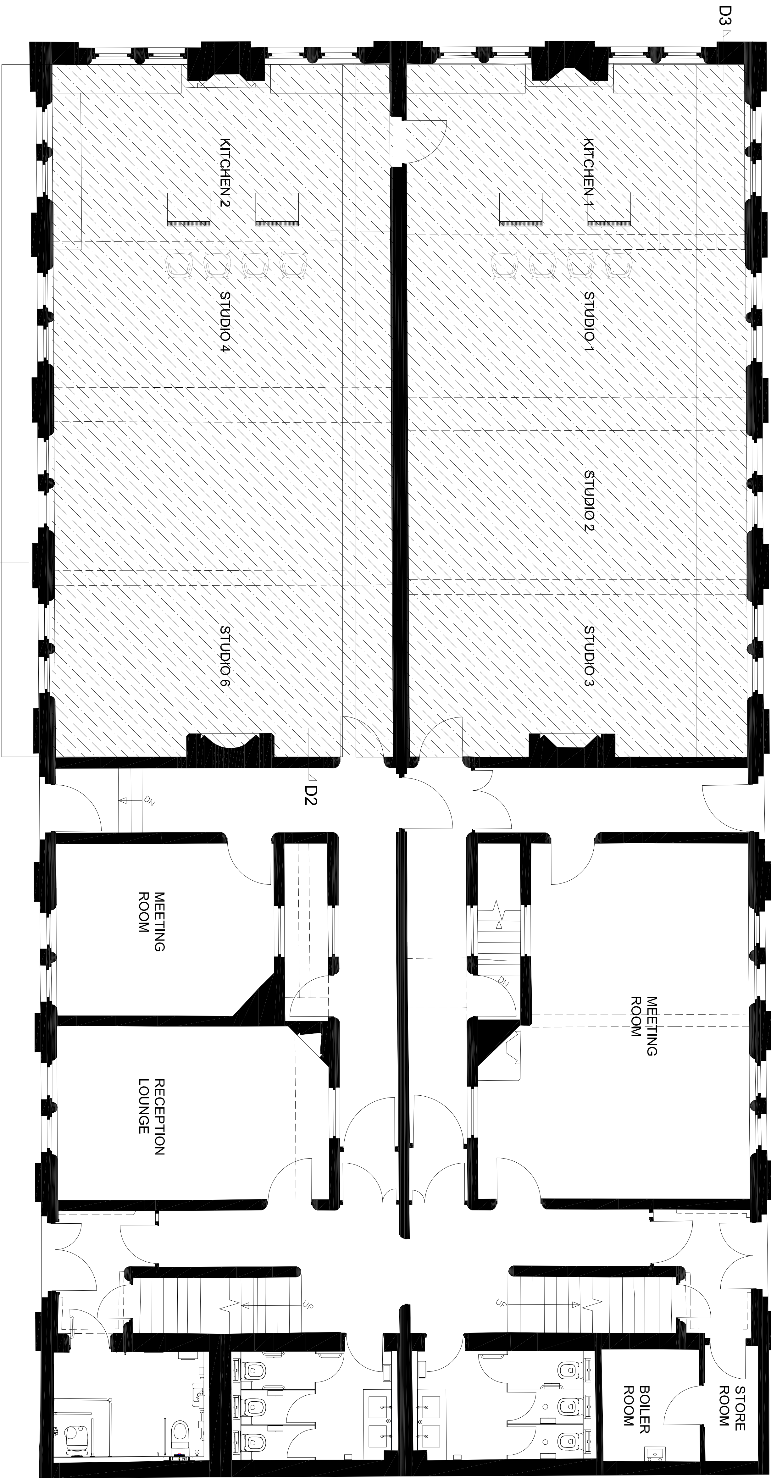
Ground Floor
