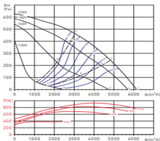
CVAB/4-6000/450N D
