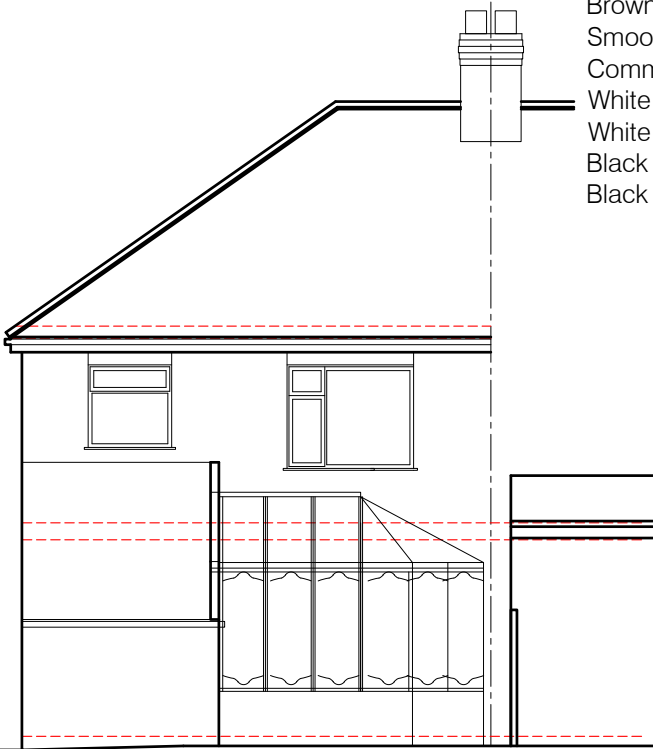
REAR ELEVATION
