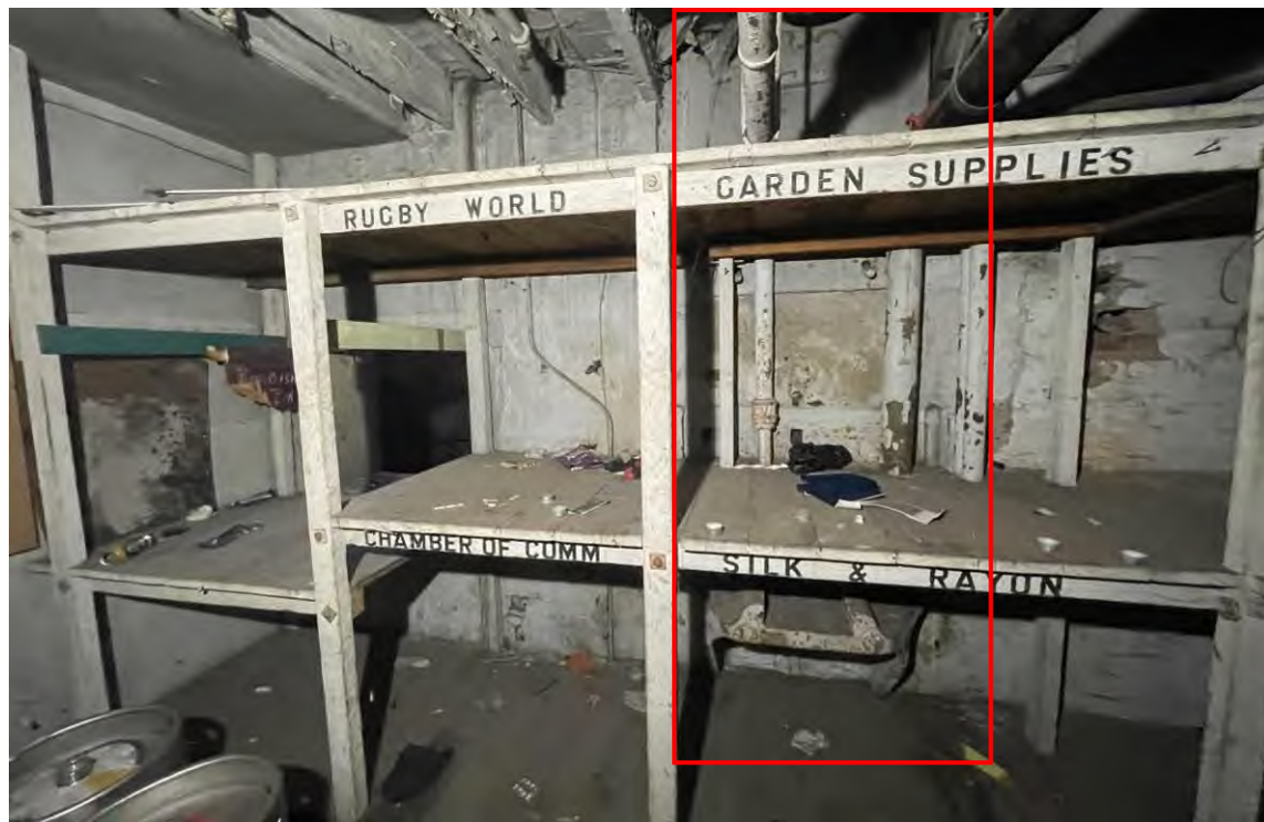
Figure 58: The 20 th century racking to the store room, showing the remnants of the original 1801 mill's engine house, which was located on the opposite (south) side of this, south wall. The large iron surrounds would have carried the original steam engine's beam.
