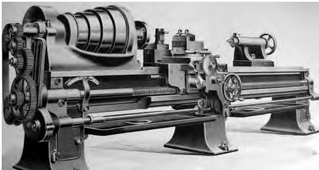
Figure 90: A drawing of the same c1902 Darling and Sellers lathe (Source: Gracesguide)
