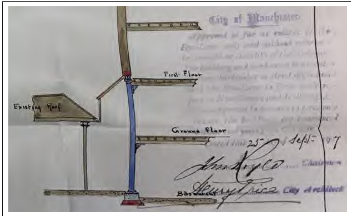
Figure 24: 1907 -.Section showing the proposed location of the lightwell between the ground and basement floor levels. (Source: Manchester Archives)
