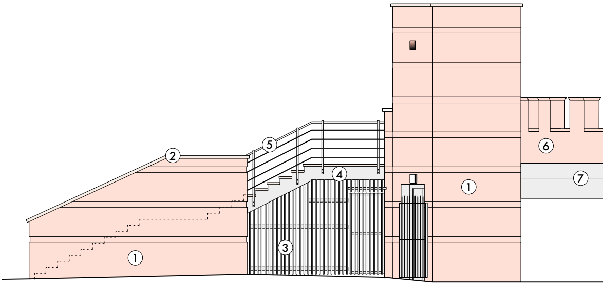
EXISTING EXTERNAL STAIR ELEVATION 1:100
