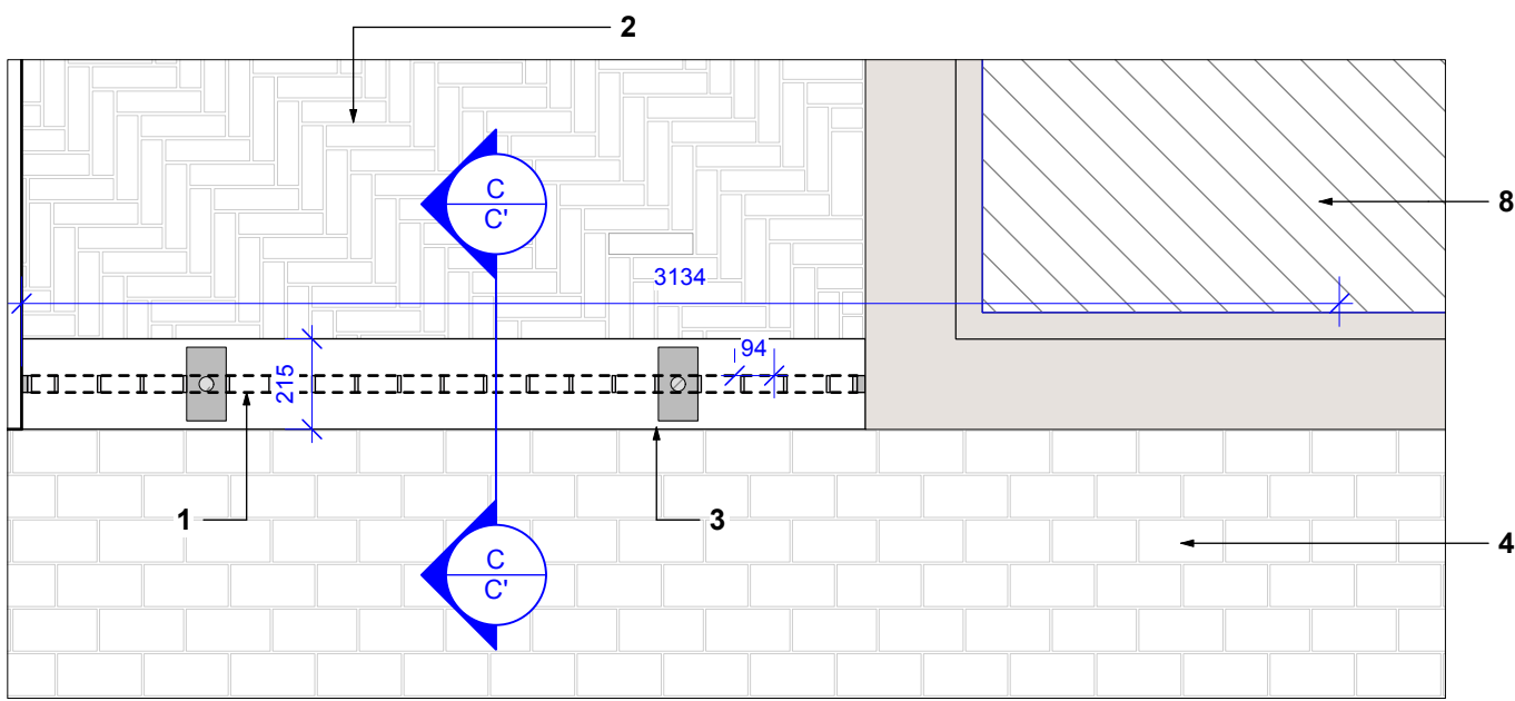
6 B6 - Brick Wall Mounted Railing - Plan Scale: 1:20
