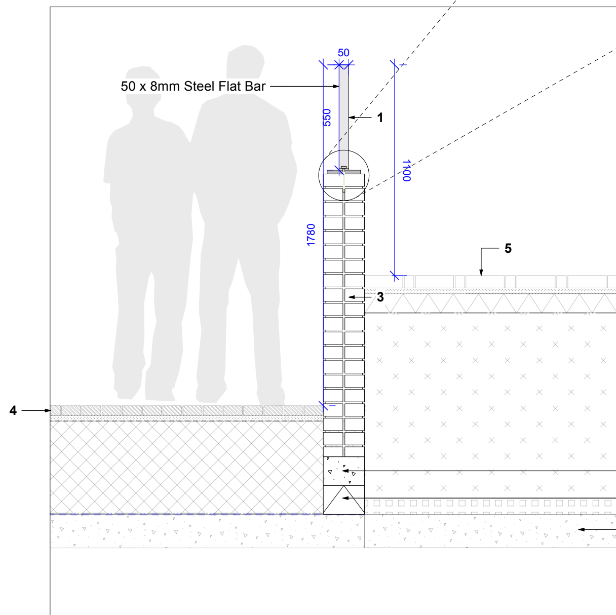
8 B6 - Brick Wall Mounted Railing - Section C-C' Scale: 1:20
