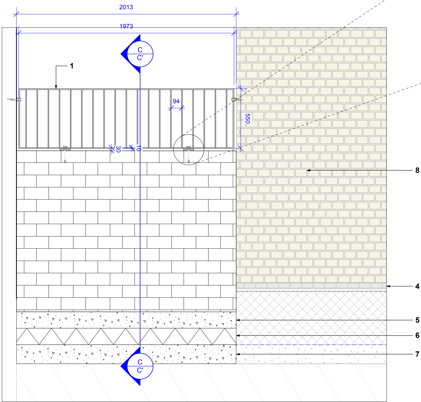
7 B6 - Brick Wall Mounted Railing - Elevation Scale: 1:20
