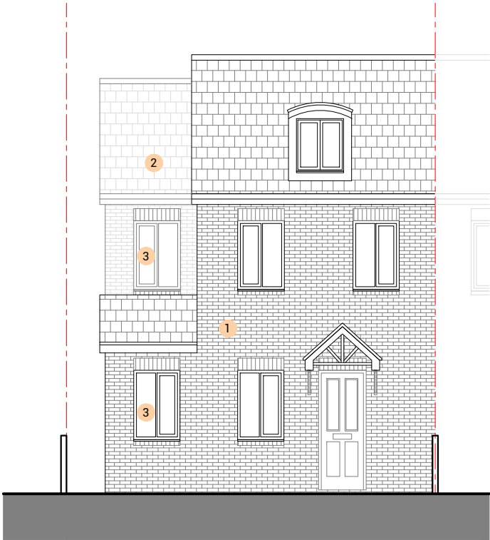
PROPOSED FRONT ELEVATION 1:100 @ A3 0m 1m 3m 5m Key 1 Brickwork to match existing 2 Roof tiles to match existing 3 PVC Window to match existing 4 Glazed Bifold Door
