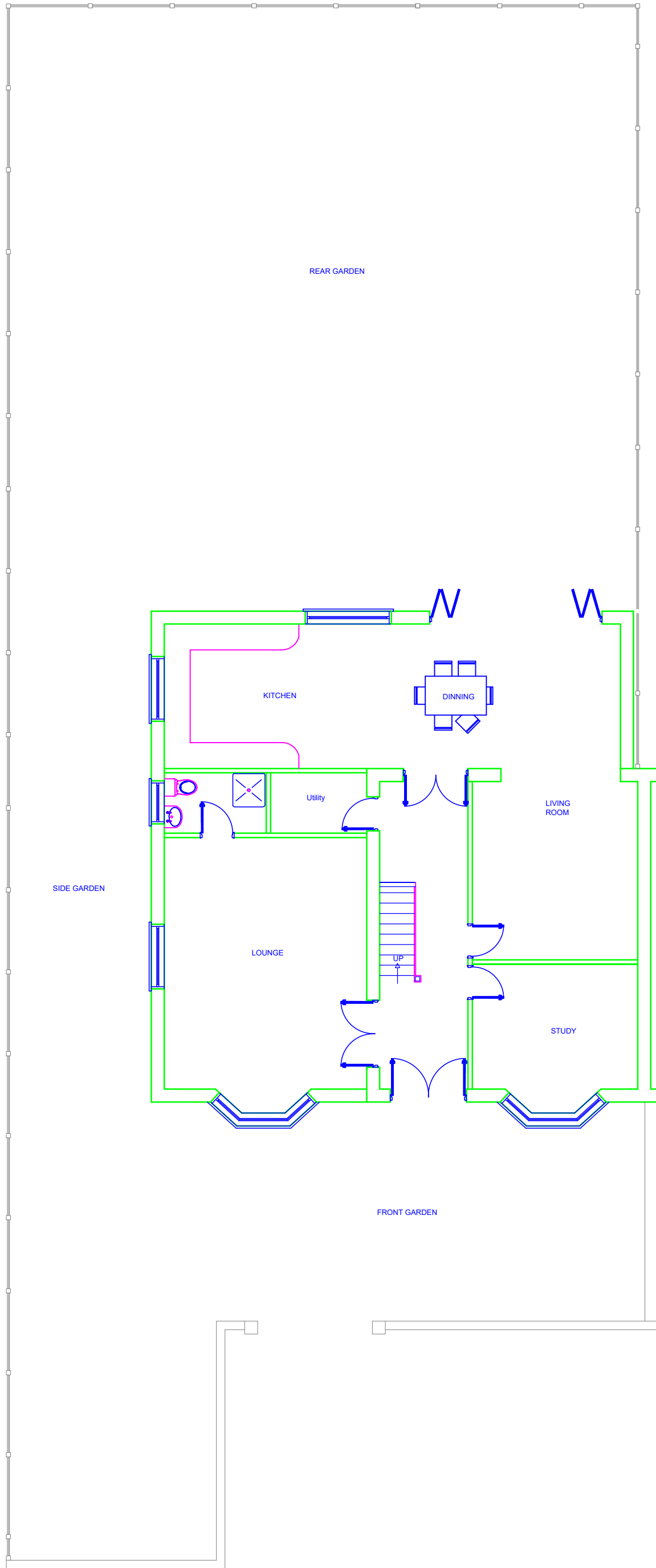
Proposed Ground Floor Plan Incl Boundary
