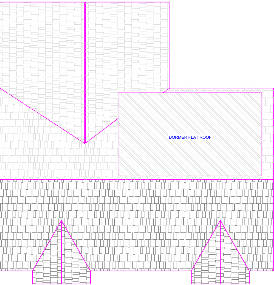
Proposed Roof Layout
