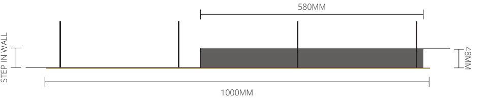
RIGHT WALL SCALE 1:10 @ A3
