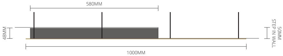
LEFT WALL SCALE 1:10 @ A3
