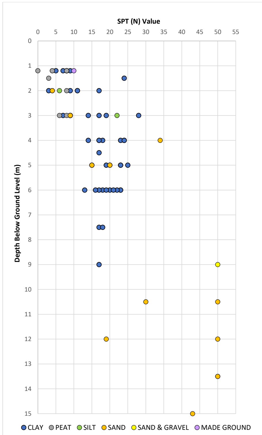
Figure 8 SPT v Depth Plot
