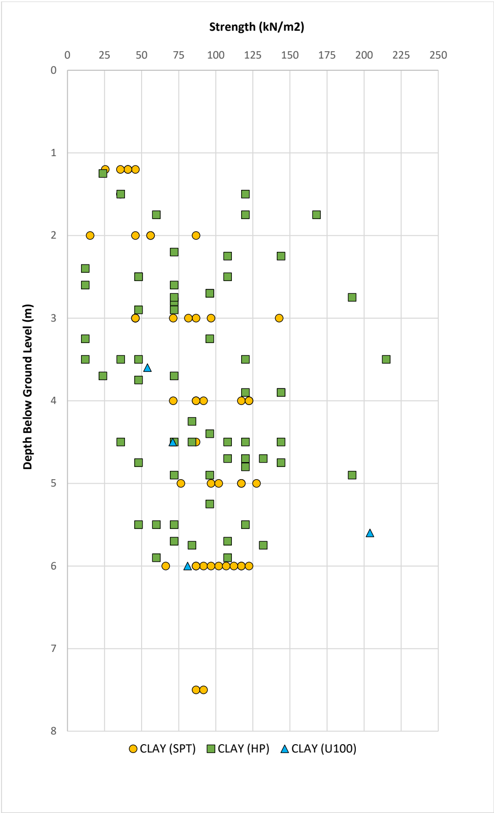
Figure 9 Strength v Depth Plot
