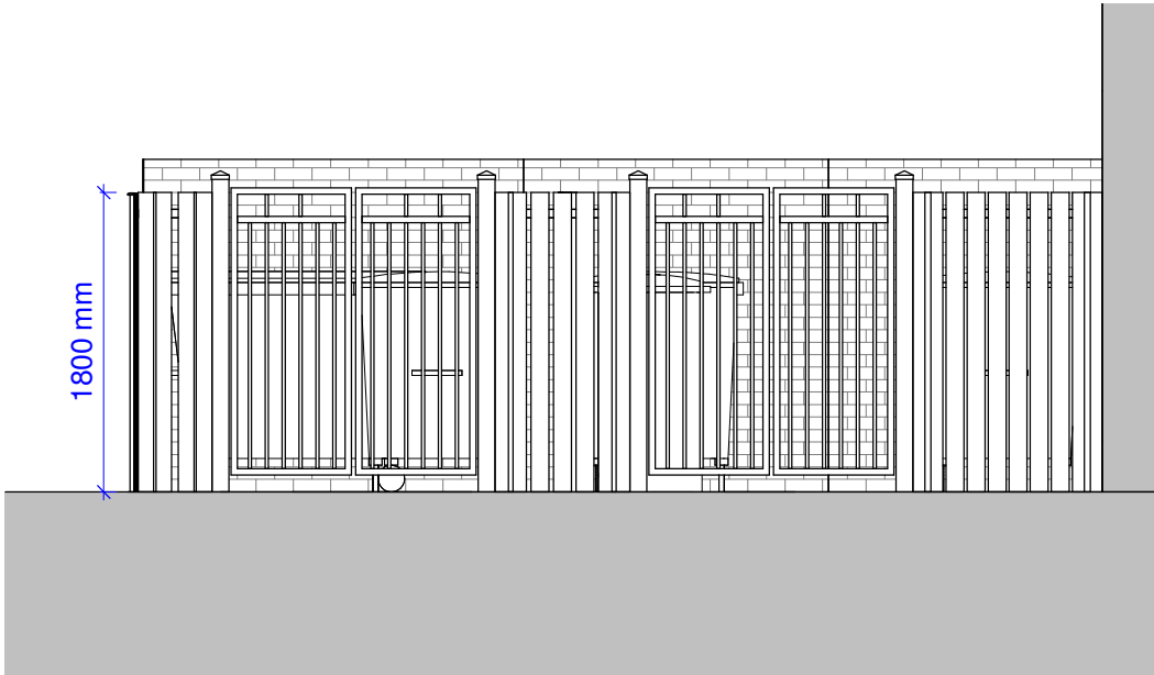
2 Proposed Bin Store_Elevation 1 : 50
