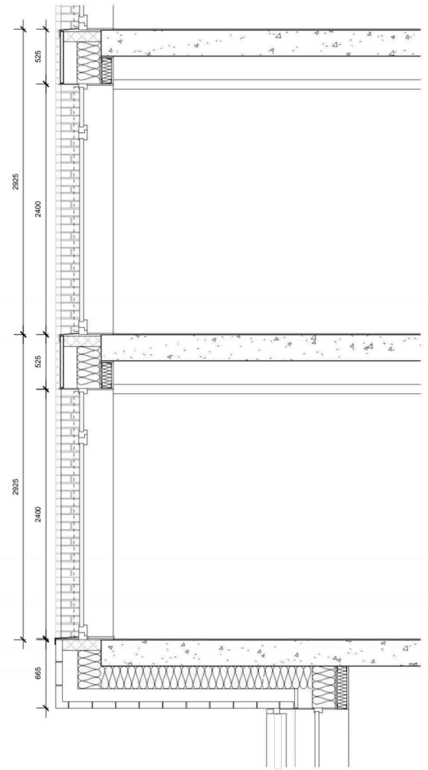
Section AA
