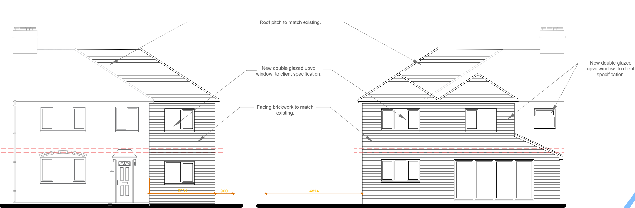
Front Elevation
