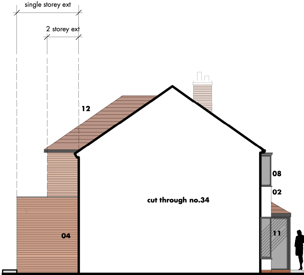
proposed side 2 elevation @ 1:100
