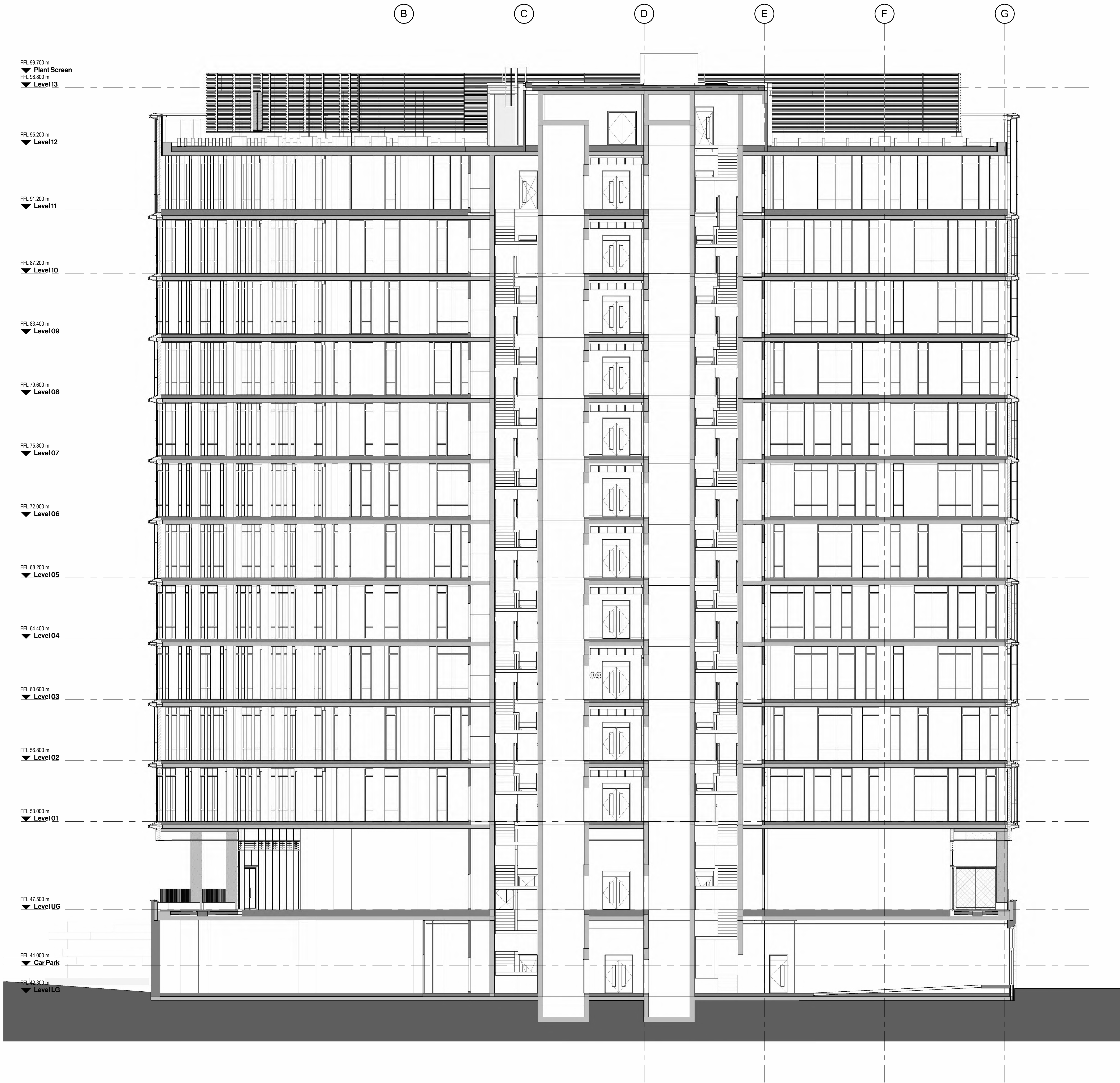
1 Section AA
