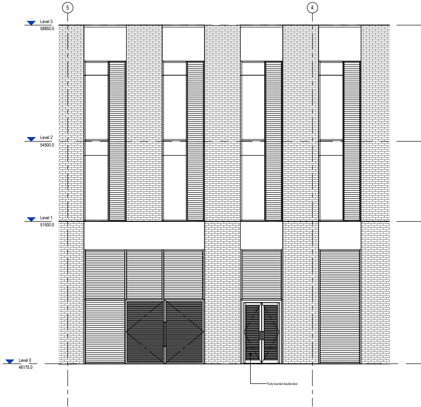
Block 1 - Consented Fire Escape - North East Elevation 1 : 50
