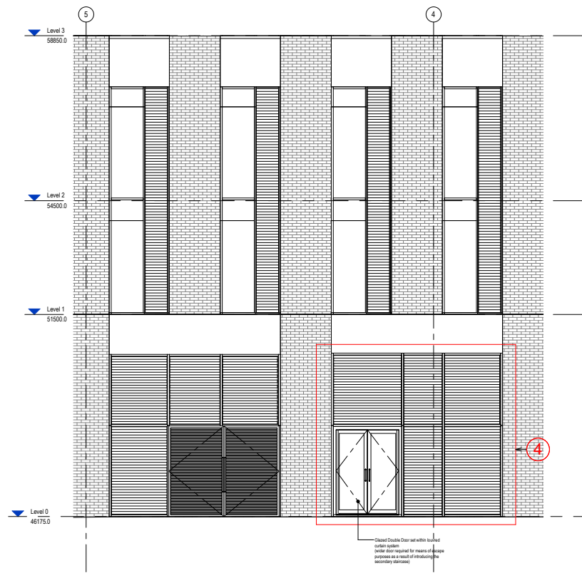
Block 1 - Proposed Fire Escape - North East Elevation 1 : 50
