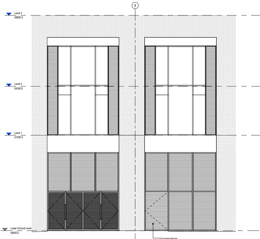
Block 2 - Consented Fire Escape - South West Elevation 1:50
