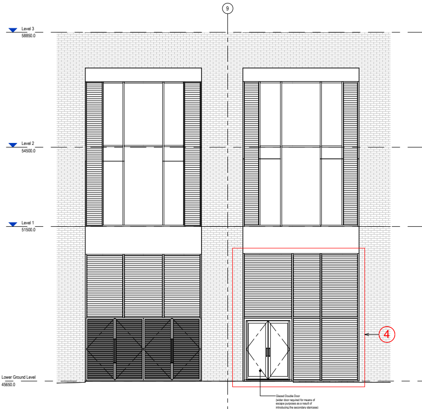
Block 2 - Proposed Fire Escape - South West Elevation 1:50
