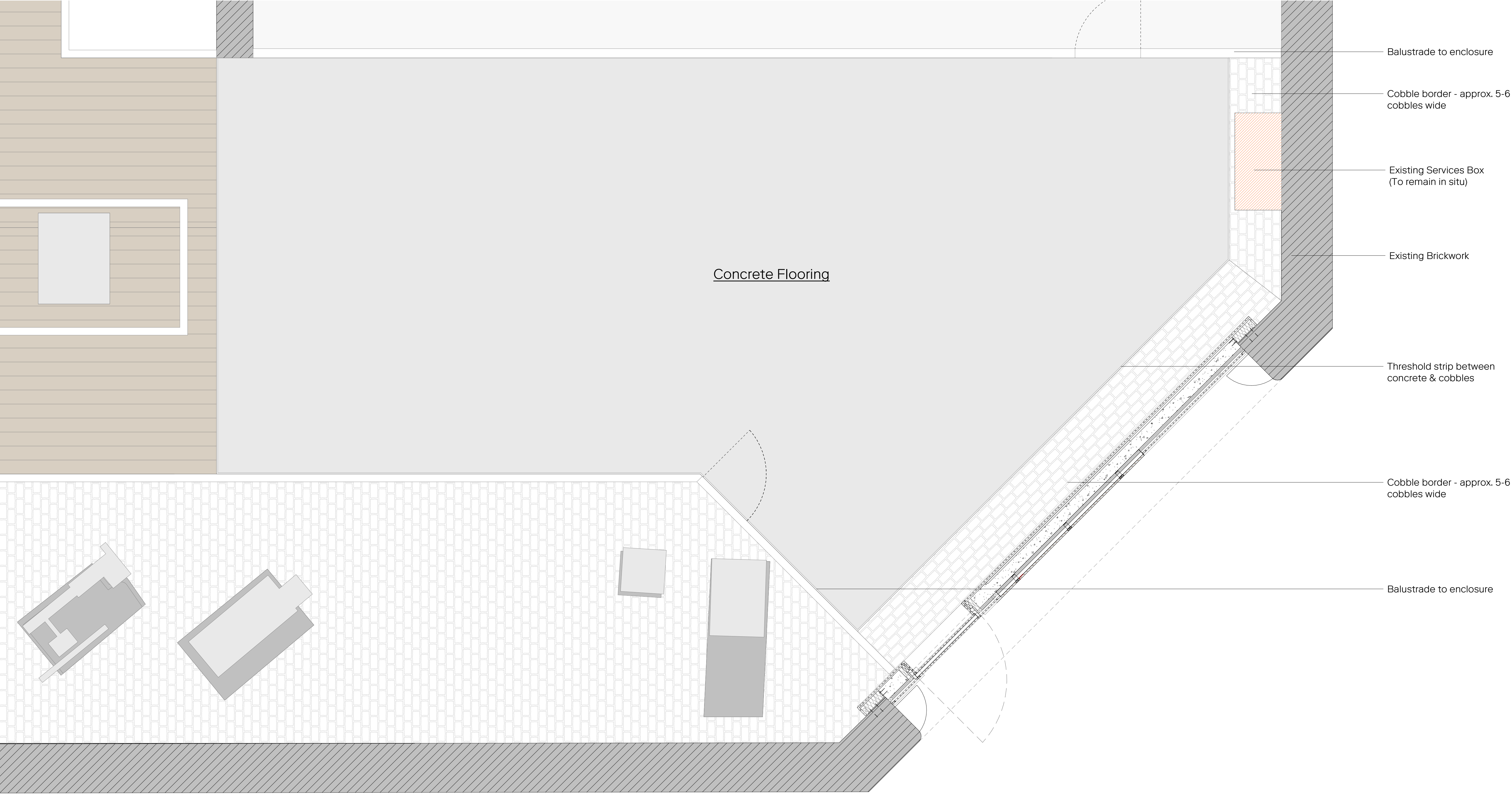
01 Junction between concrete floor & historic brick walls 1 : 25 @ A1
