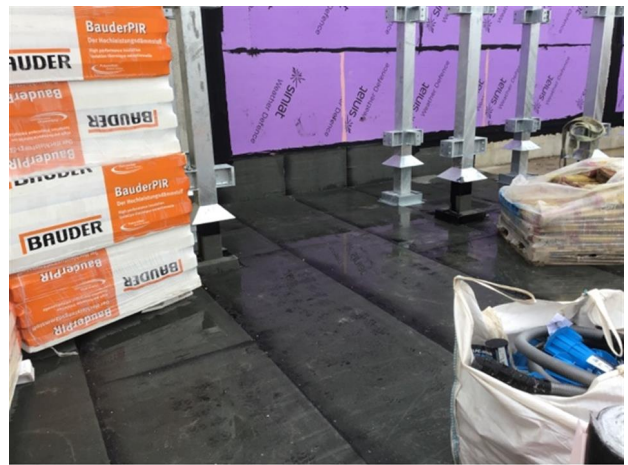
Photo 6 - View of AVCL to level 9 section 1
