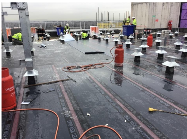
Photo 1 - View of level 9 section 1
