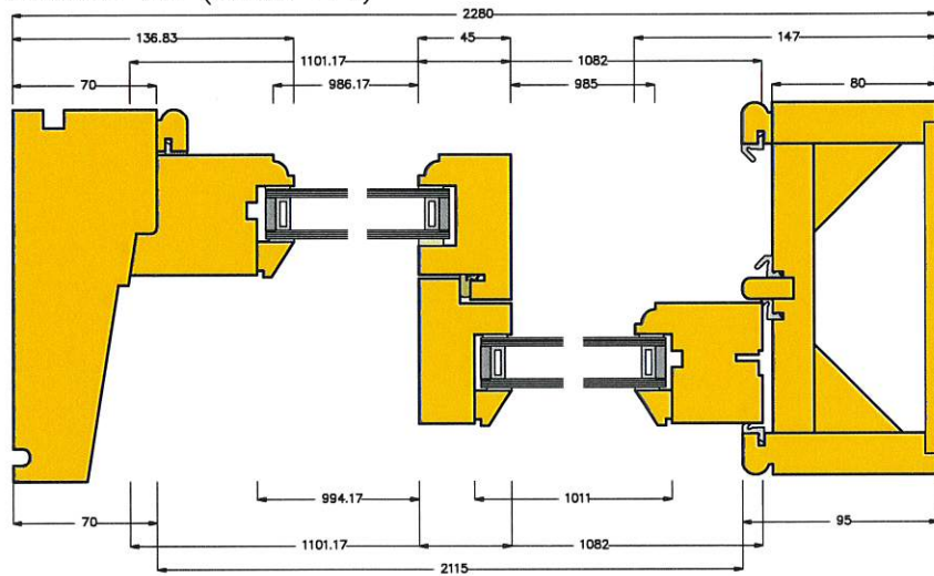
Section C4 (scale 1:4)
