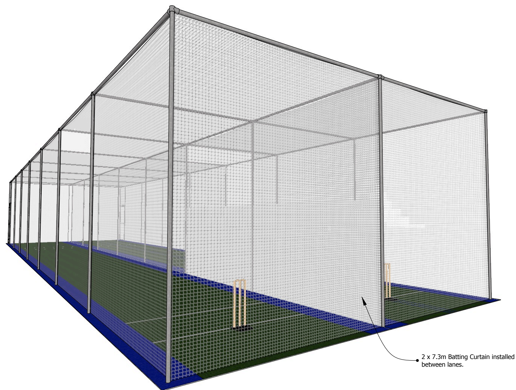
REAR PERSPECTIVE
