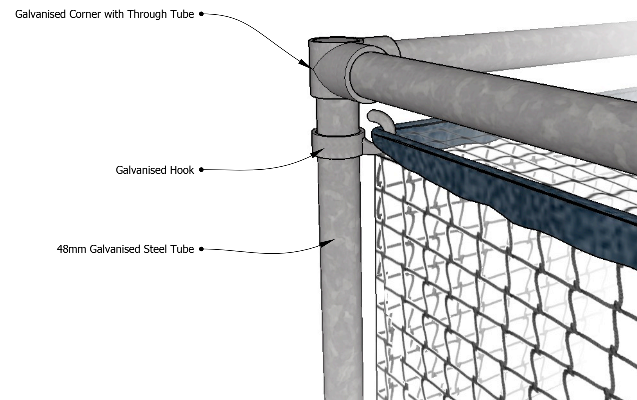
CAGE POST DETAIL
