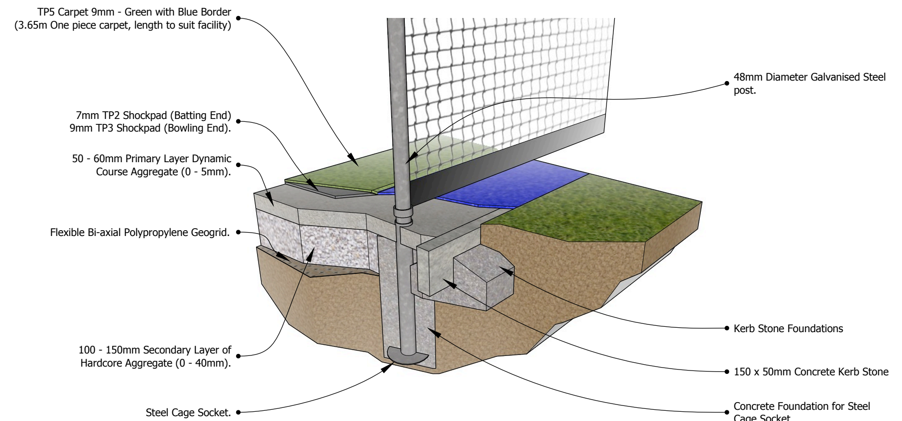
CAGE POST INSTALLATION
