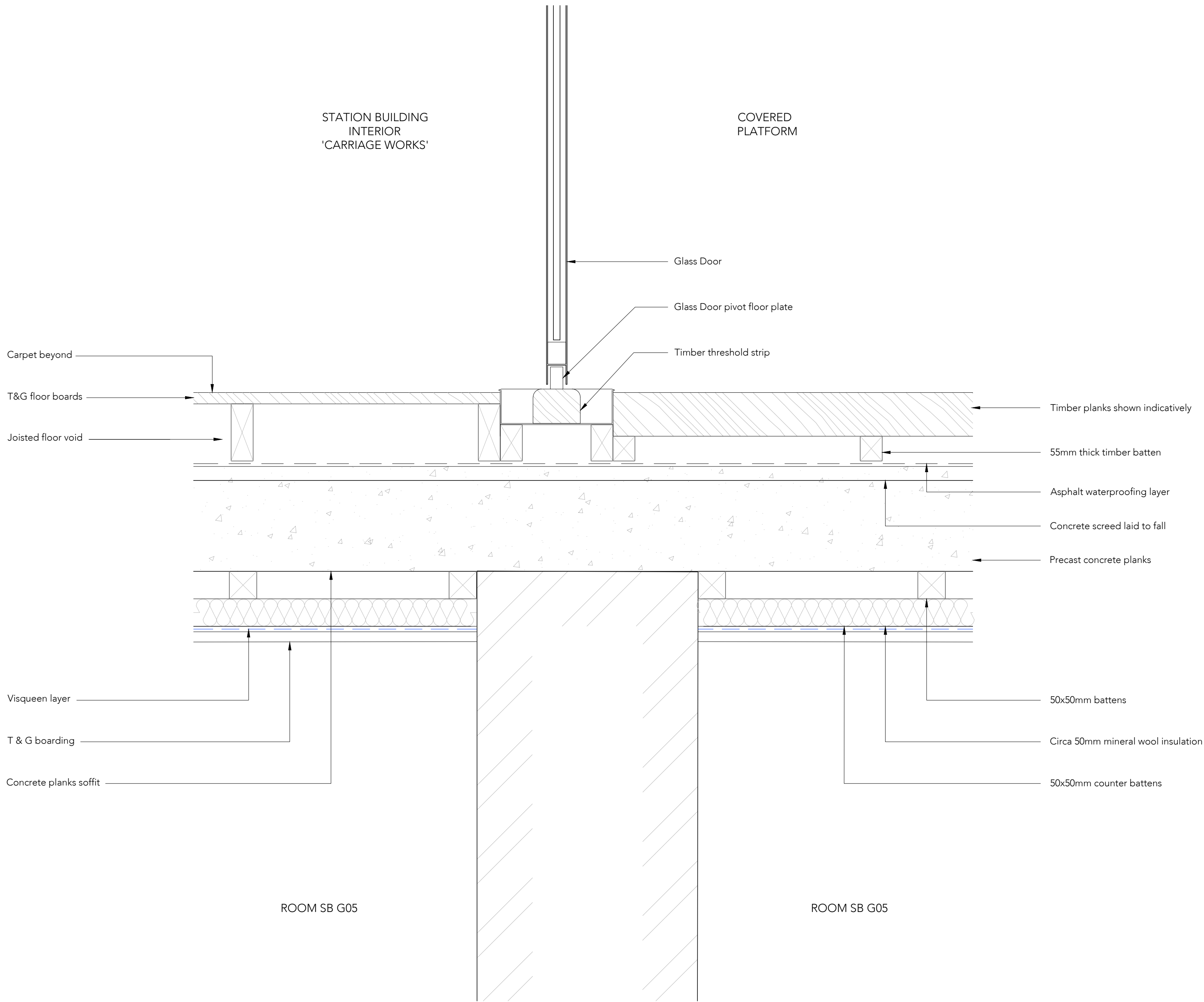
Typical Detail Through Glass Door Threshold K-K as Existing Scale 1:5
