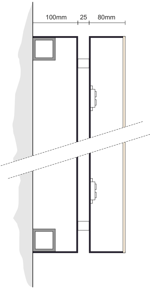
Section through Scale 1:5 @ A3
