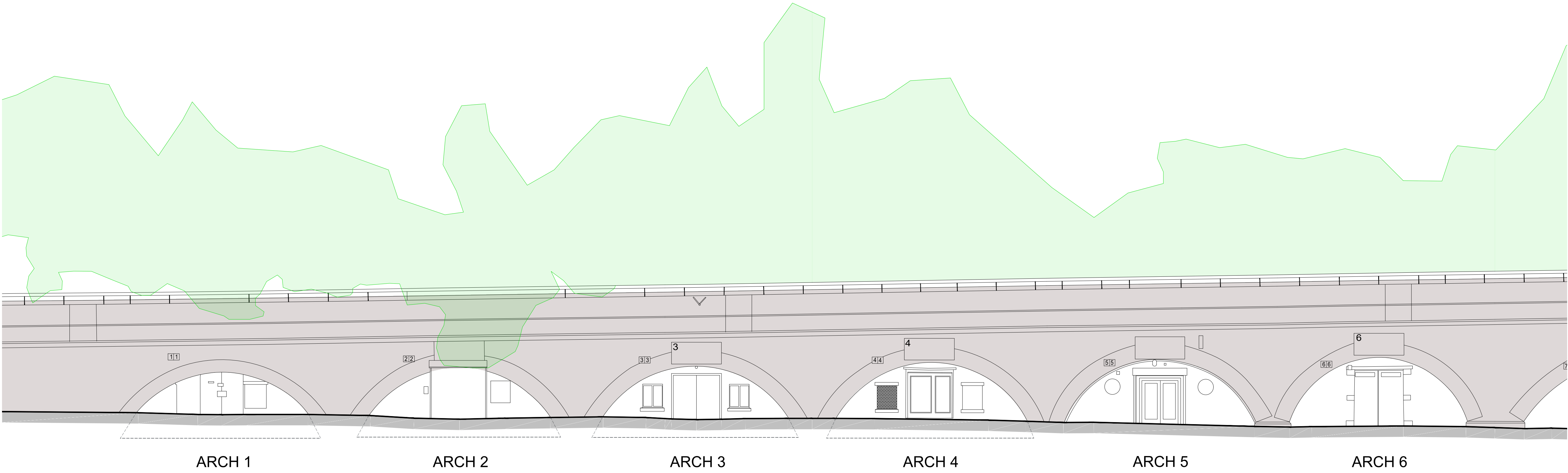
EXISTING ELEVATIONS ARCHES 1-6
