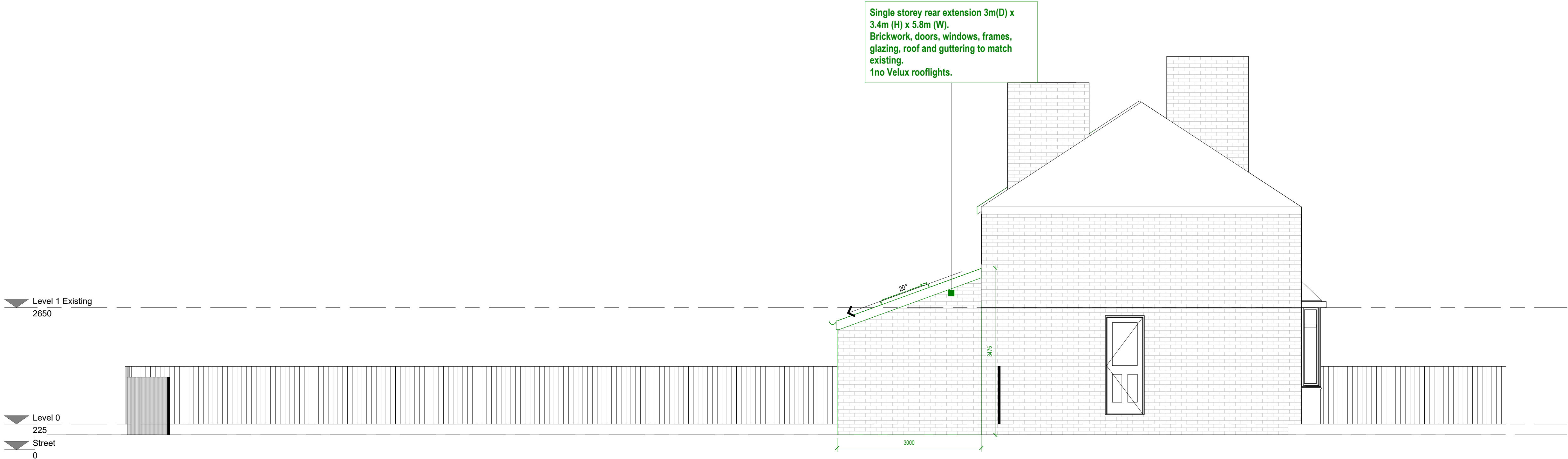
Proposed Side 1 Elevation 1 : 50
