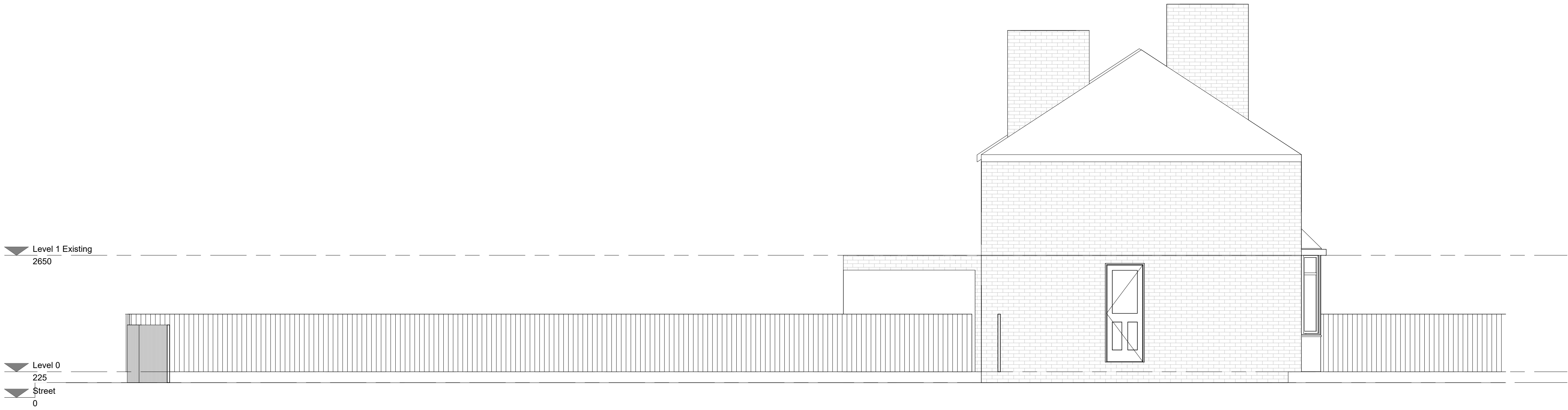
Existing Side 1 Elevation 1 : 50
