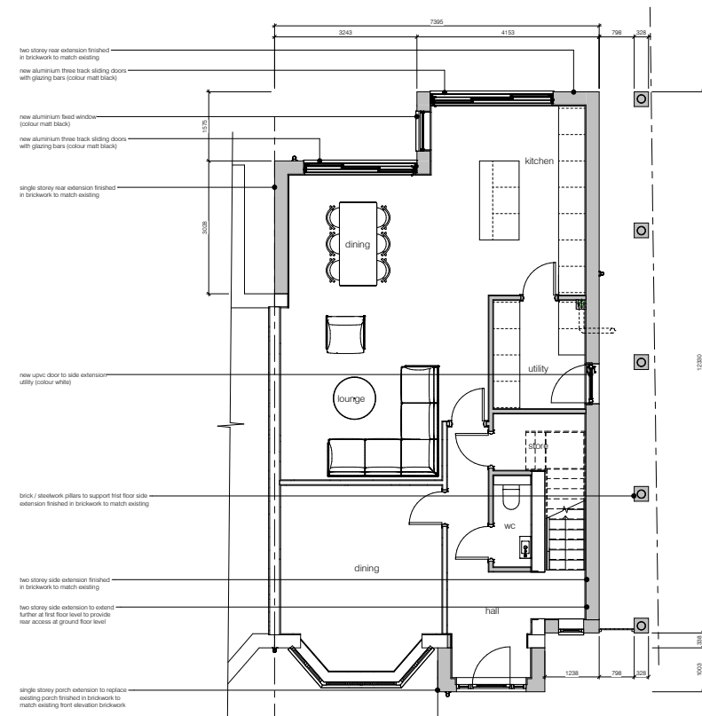
00 proposed ground floor 1 : 50
