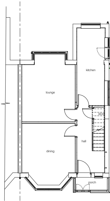
00 existing ground floor 1 : 50
