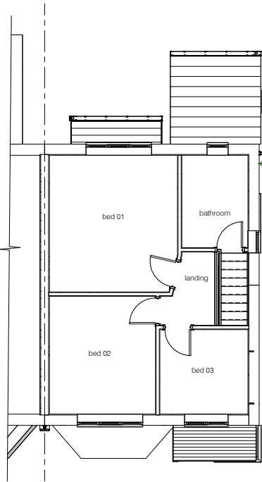
01 existing first floor 1 : 50
