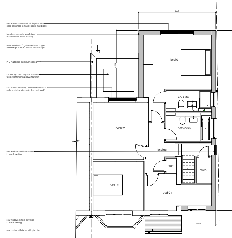
01 proposed first floor 1 : 50
