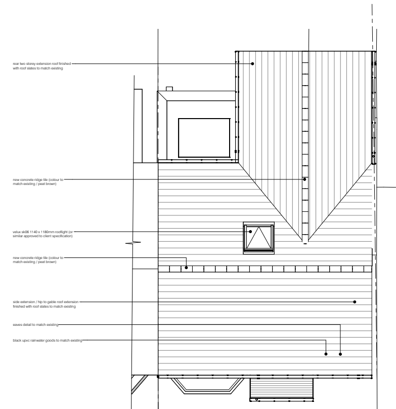
proposed roof plan 1 : 50
