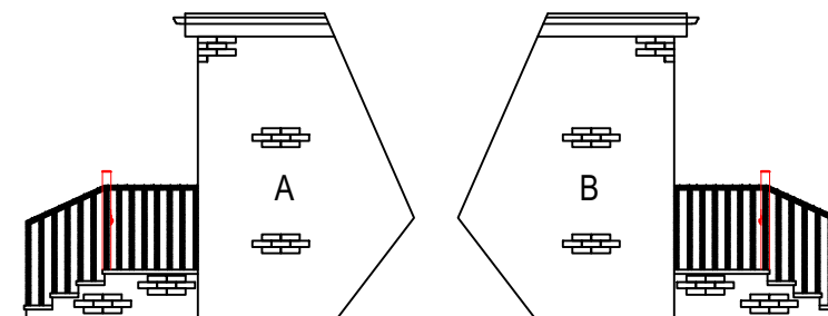
PROPOSED SIDE ELEVATIONS A & B
