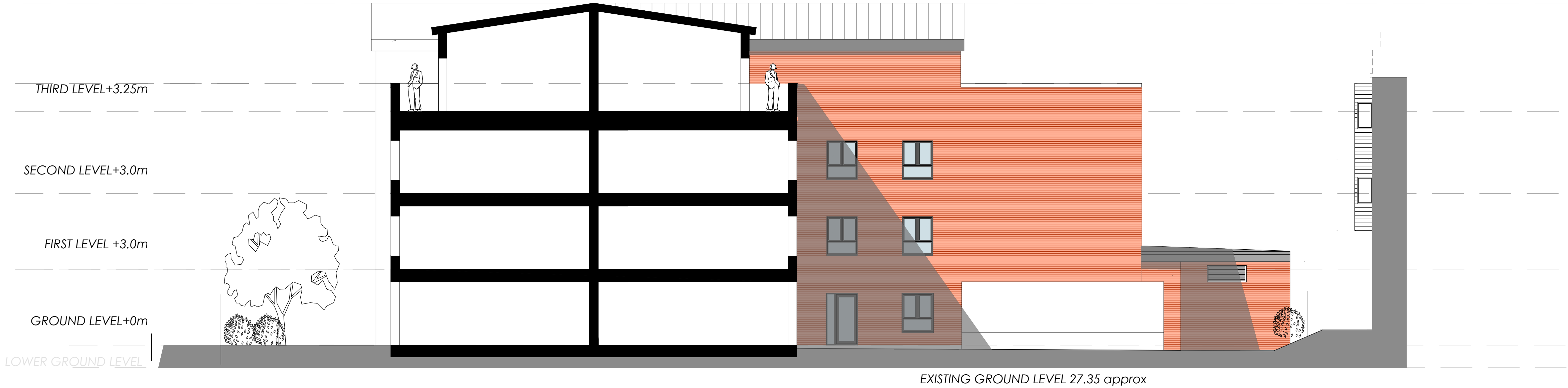
WESTERN REAR COURTYARD ELEVATION
