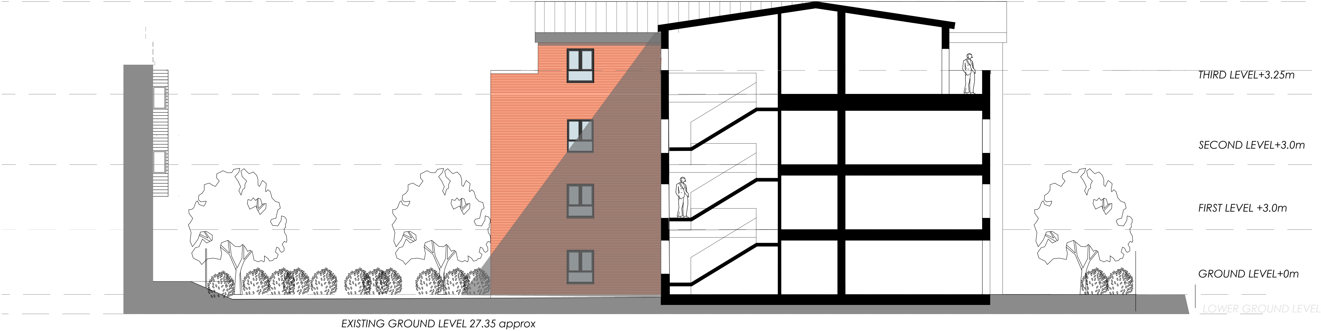
EASTERN REAR COURTYARD ELEVATION
