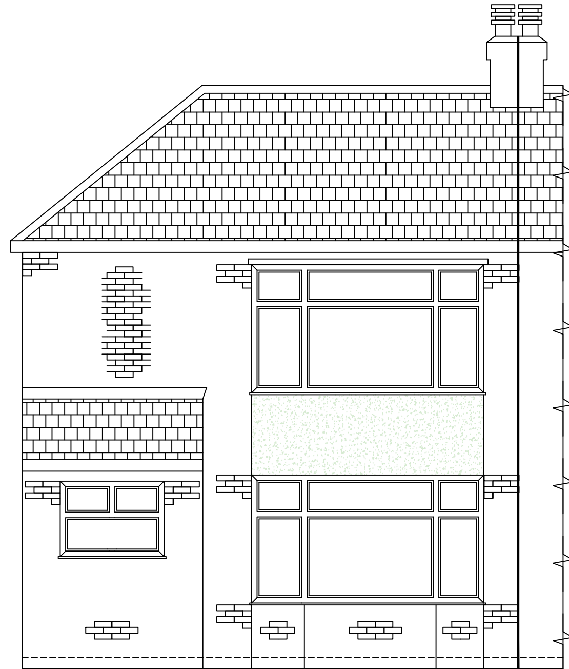
EXISTING REAR ELEVATION - REF 003
