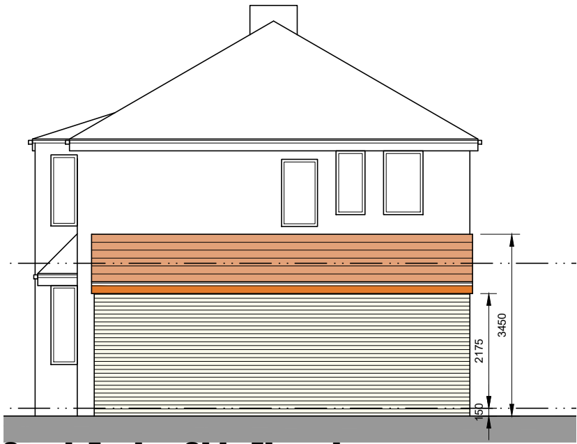
South Facing Side Elevation
