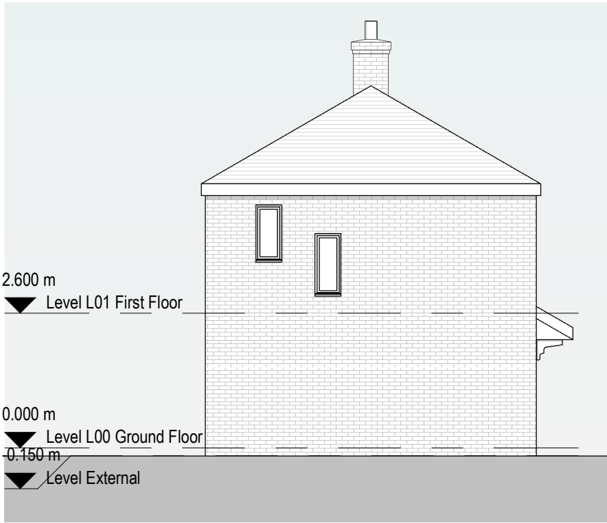
4 Existing West Elevation 1 : 100
