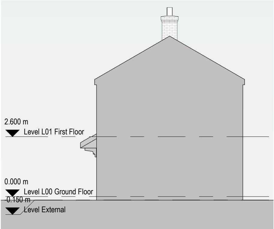
2 Existing East Elevation 1 : 100
