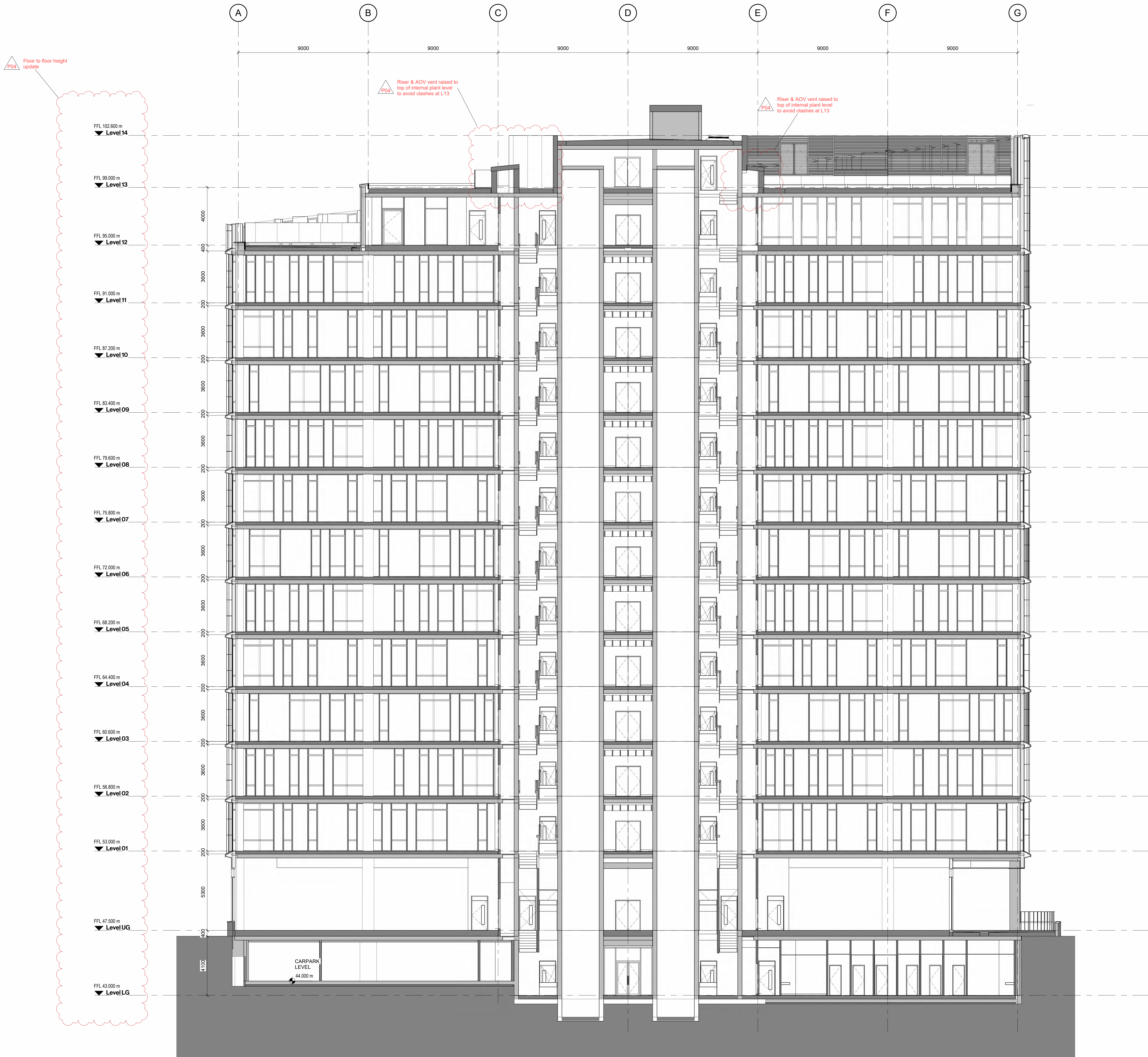
1 Section - AA
