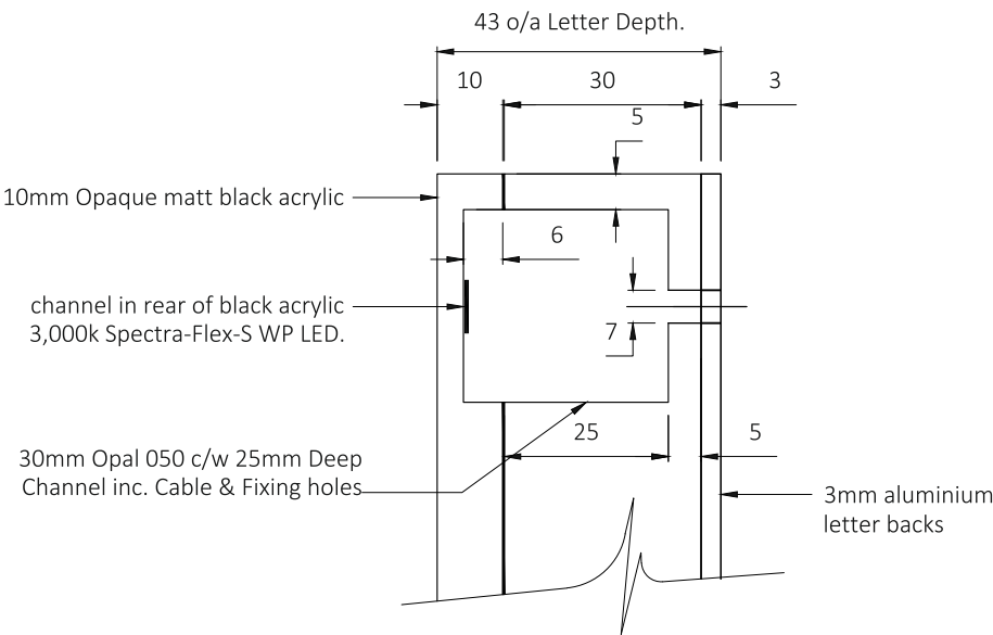
Item B: Fascia Letters- Scale 1:15 2-off Digitally Printed Opaque Vinyl Patches. Note: - Applied to Awning Valance.
