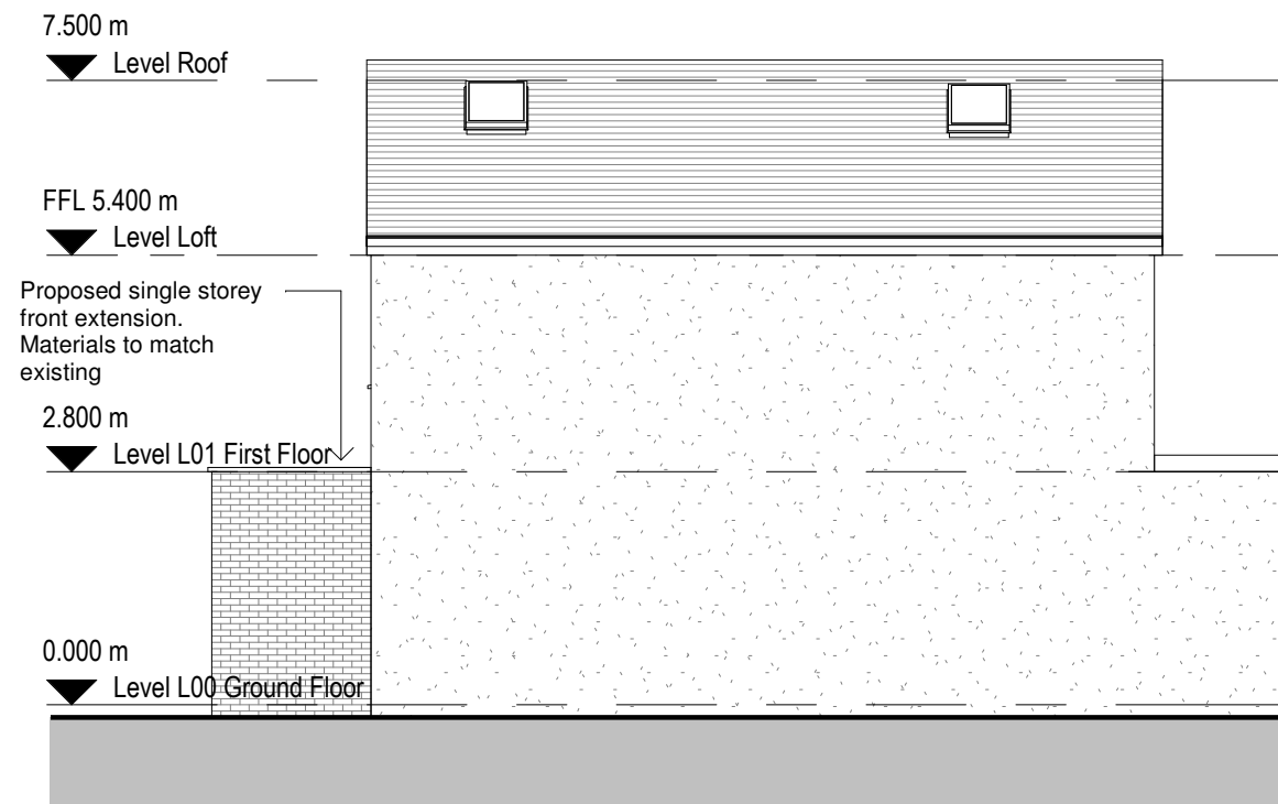
3 Proposed West Elevation 1 : 100
