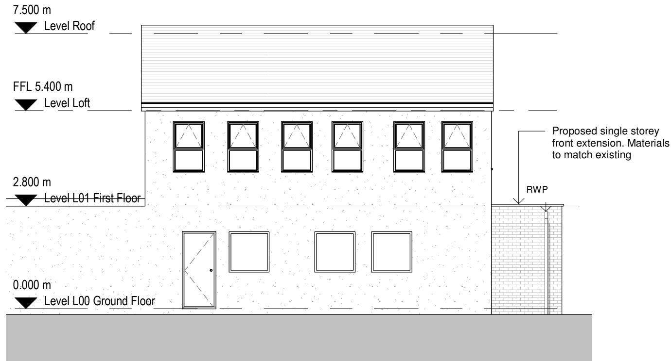
2 Proposed East Elevation 1 : 100
