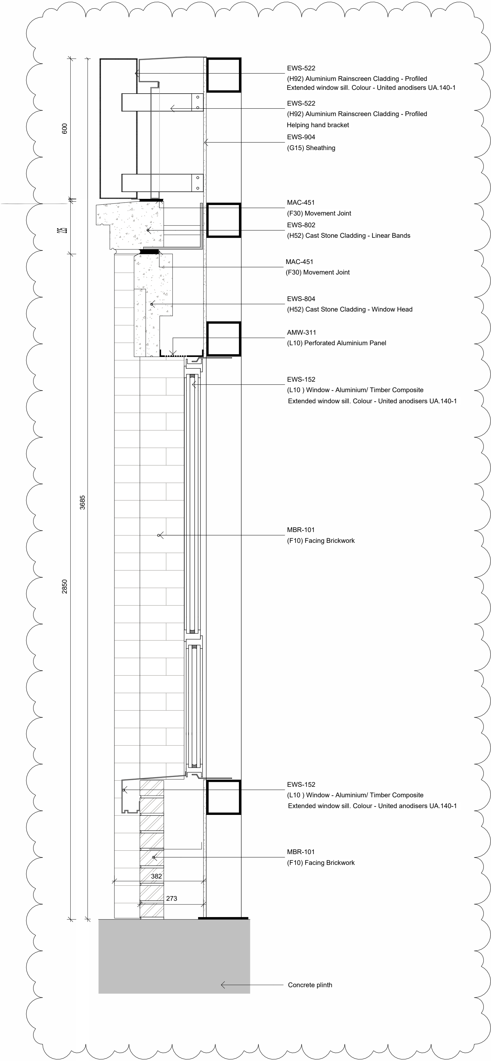
Typical Section - VMU 1 : 10
