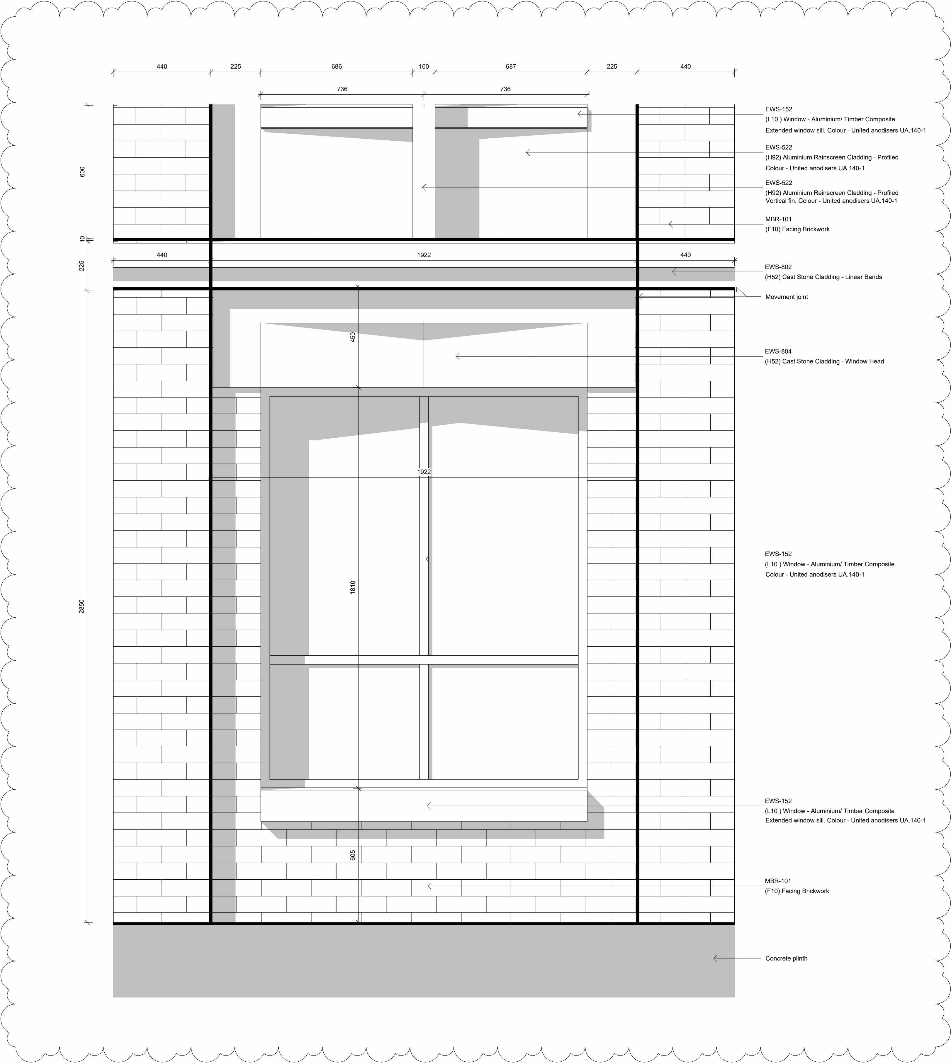
Typical Bay - Brickwork and Architectural Wetcast - VMU 1 : 10
