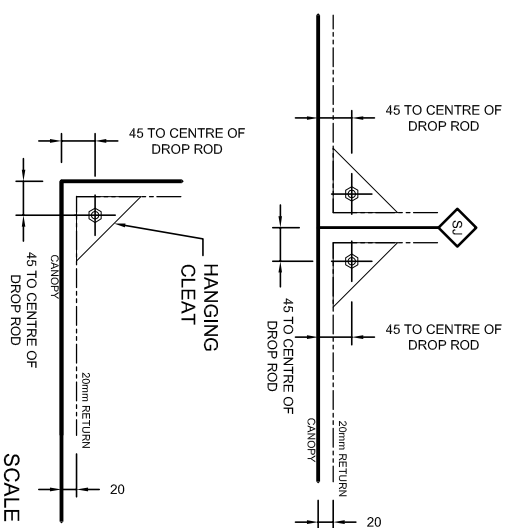
HANGING CLEAT POSITION:
