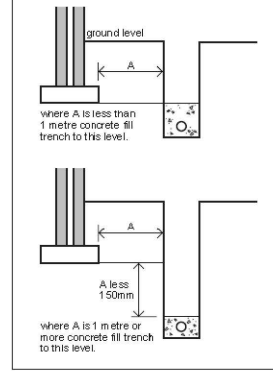
Diagram 8 Pipe runs near buildings
