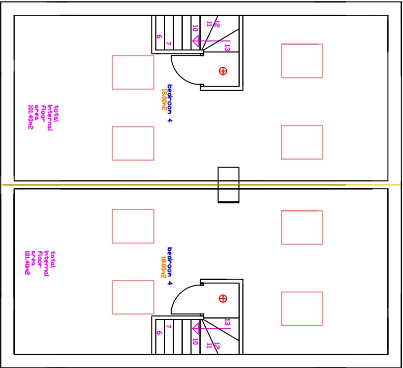
PROPOSED LOFT FLOOR 1:100
