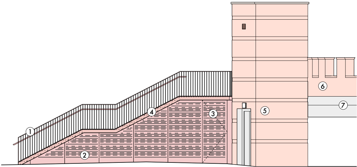
PROPOSED EXTERNAL STAIR - OPTION 1 ELEVATION 1:100
