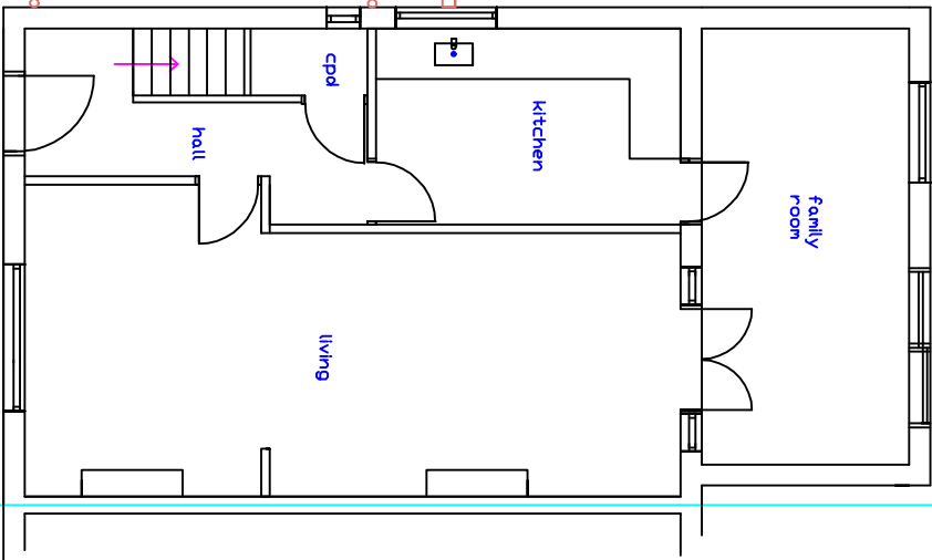
EXISTING GROUND FLOOR 1:100
