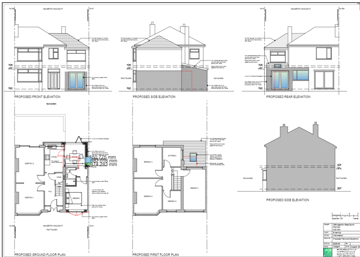
Figure 1. Proposed plans and elevations
