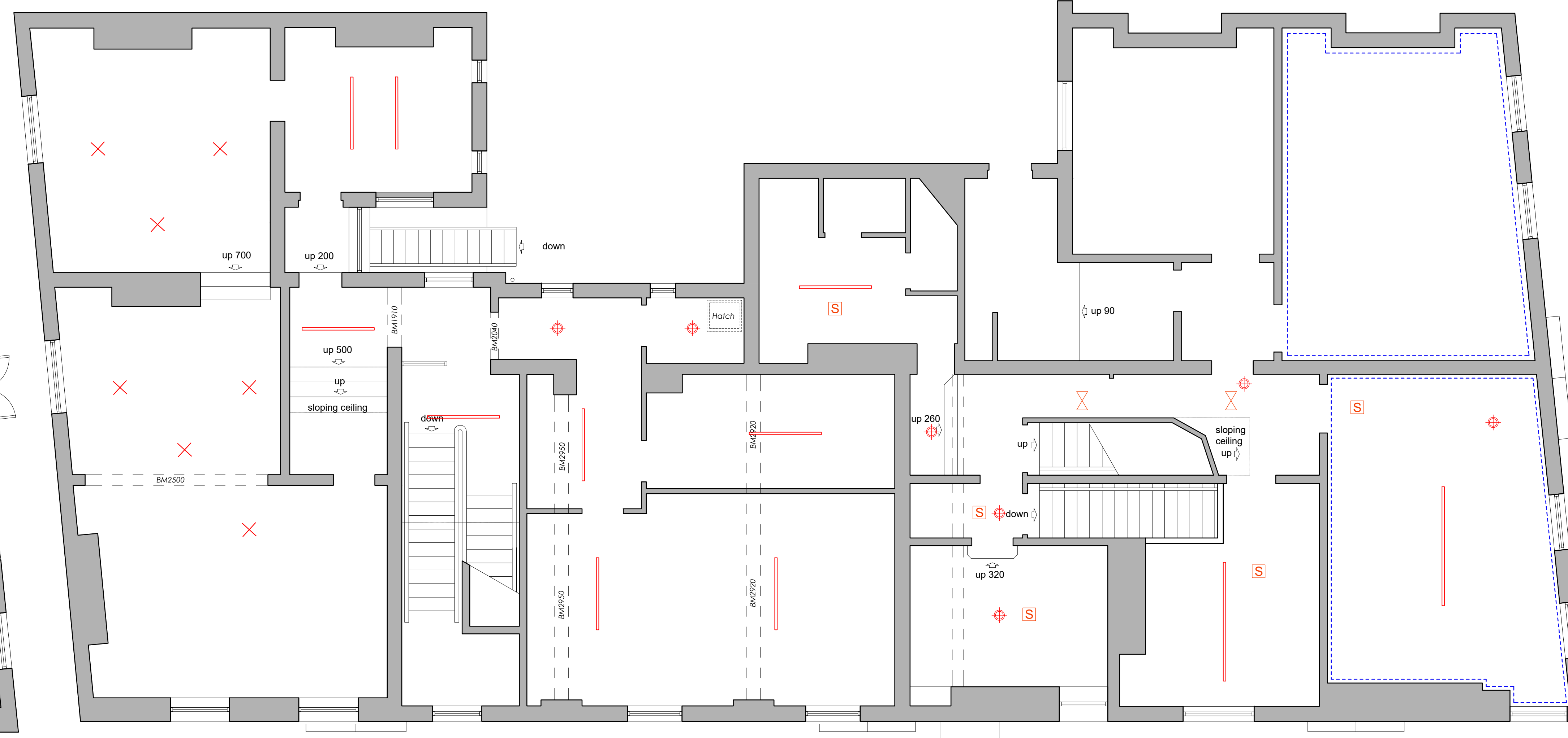
FIRST FLOOR CEILING PLAN AS EXISTING
