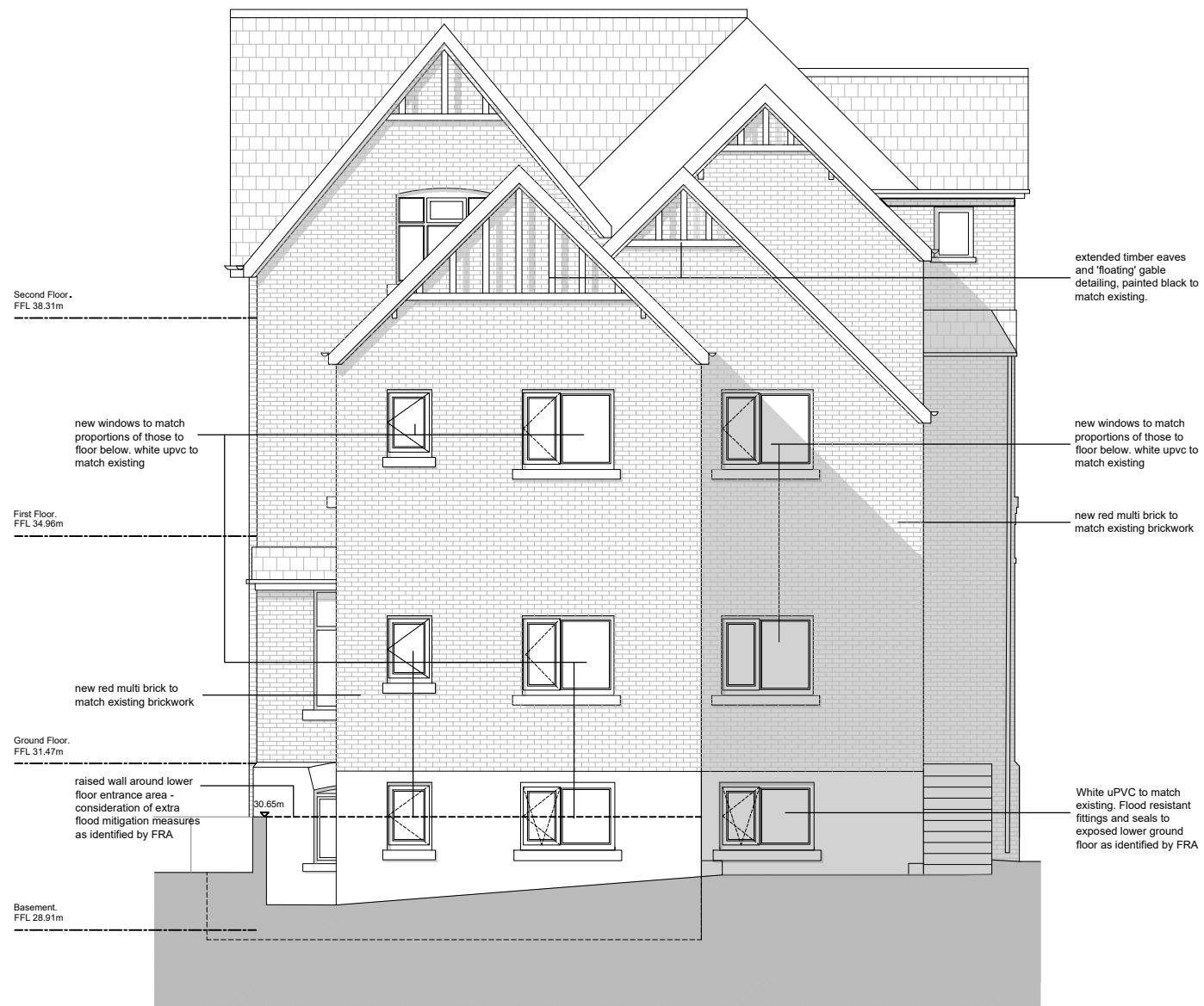
East (Rear) Elevation
