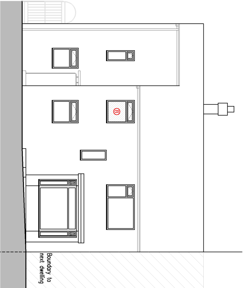
Proposed West Elevation (Principal)
