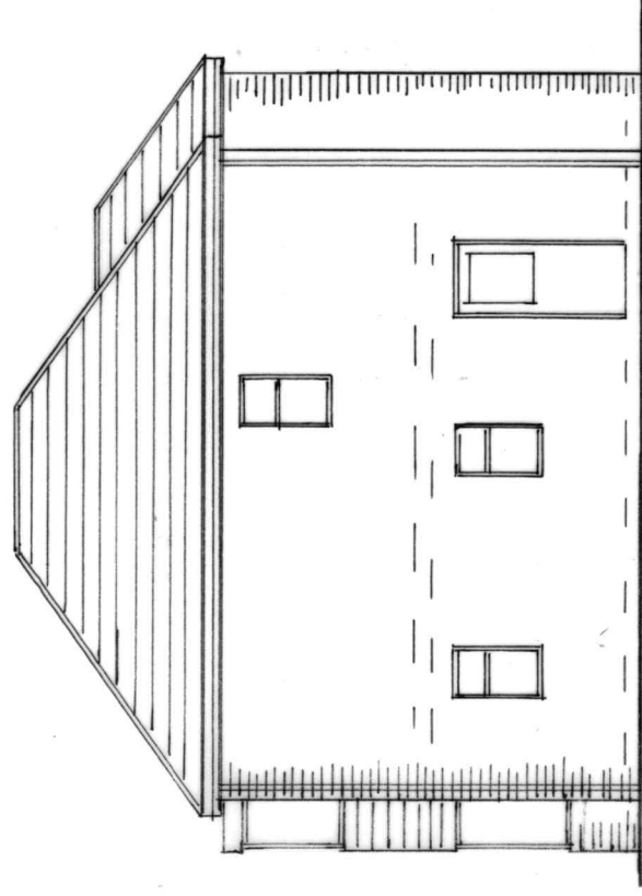
SIDE ELEVATION
