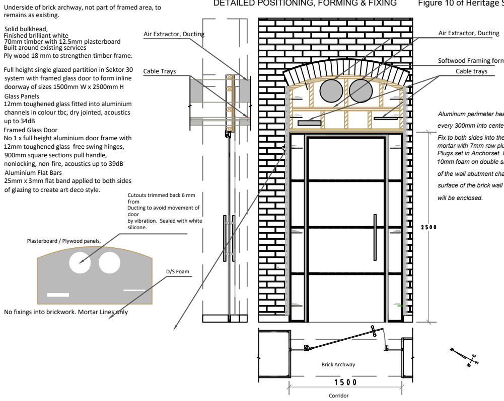
EXTERNAL VIEW 1:20@A3 Second Floor Partition 2 DETAILED POSITIONING, FORMING & FIXING Figure 10 of Heritage Statement
