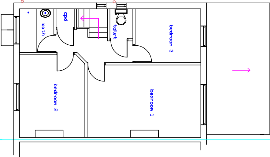
EXISTING FIRST FLOOR 1:100
