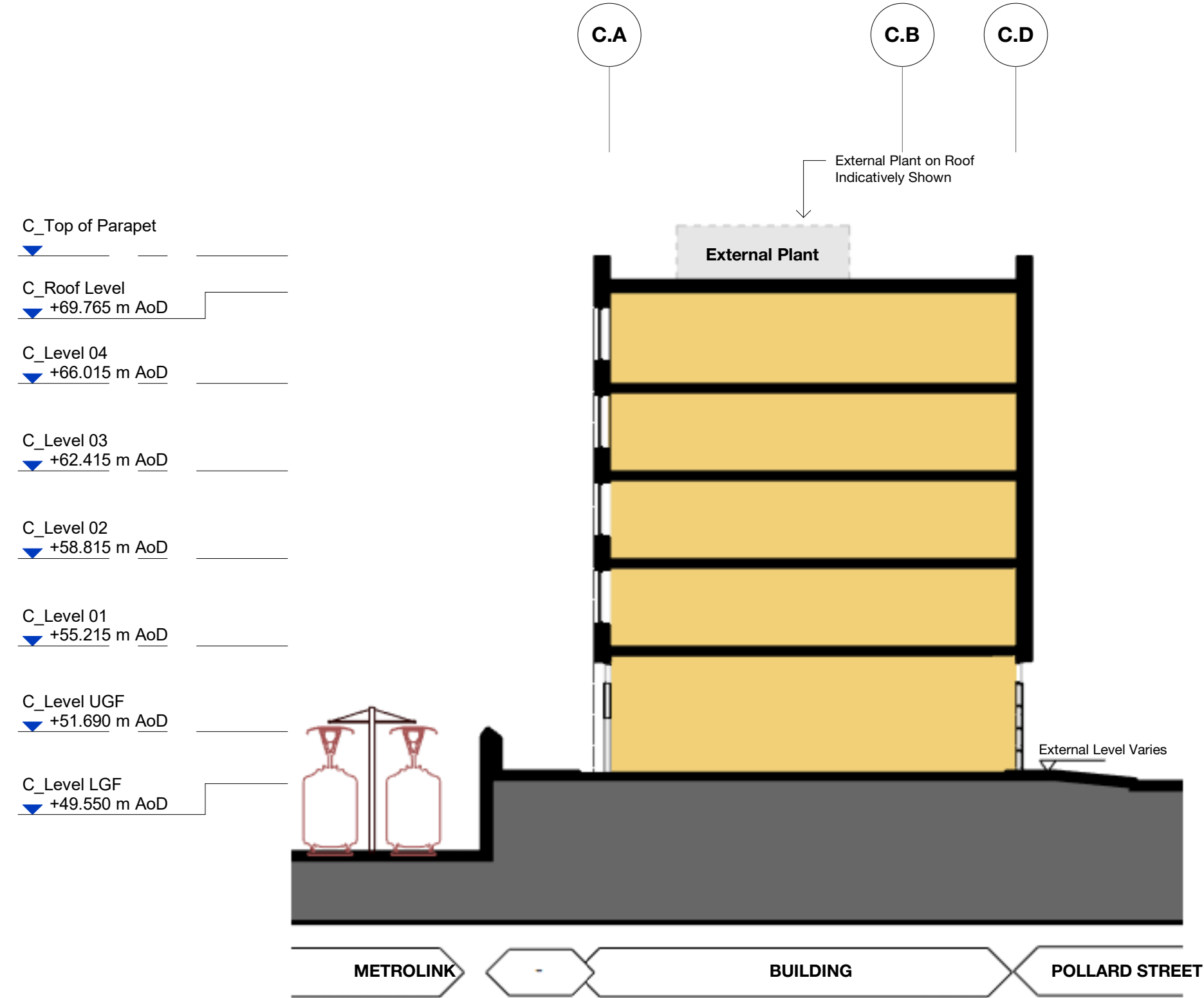
Building C - Proposed Section AA 1 : 200
