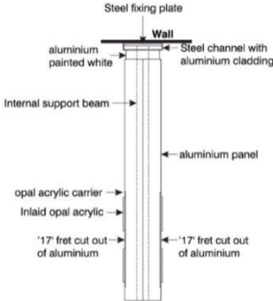
Plan View (Cross section A - A)
